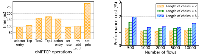
(a) Overhead of the main operators of eMPTCP.
