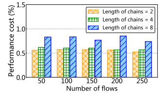
(b) Overhead of eMPTCP with different length of policy chains.
