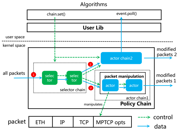
Fig. 2: eMPTCP overview.
