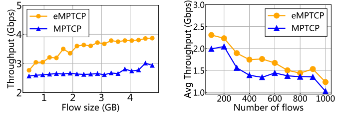
(a) Comparison of throughput with traffic scheduler. (b) Comparison of avg throughput for multi flows.
