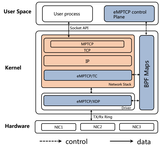
Fig. 1: eMPTCP and the networking stack.
